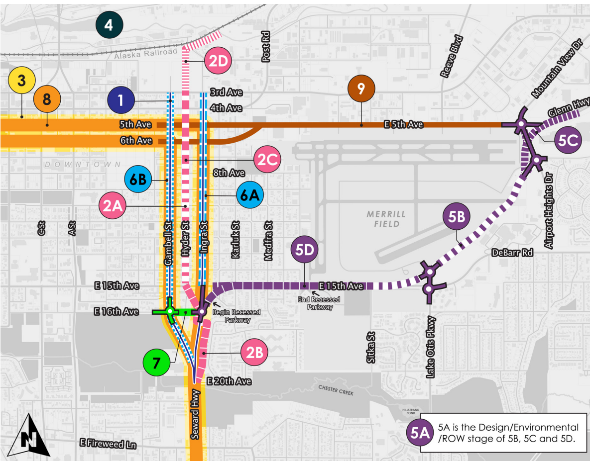
Figure 27: Phasing Plan: Overview Map.
