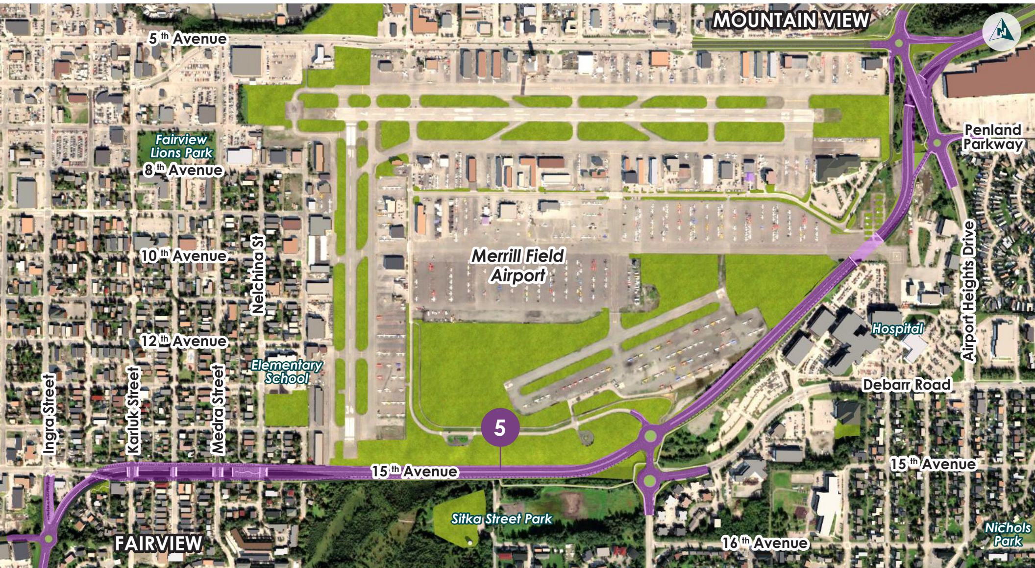
Figure 40: A Plan View of the Entire Recommended Fairview Bypass
