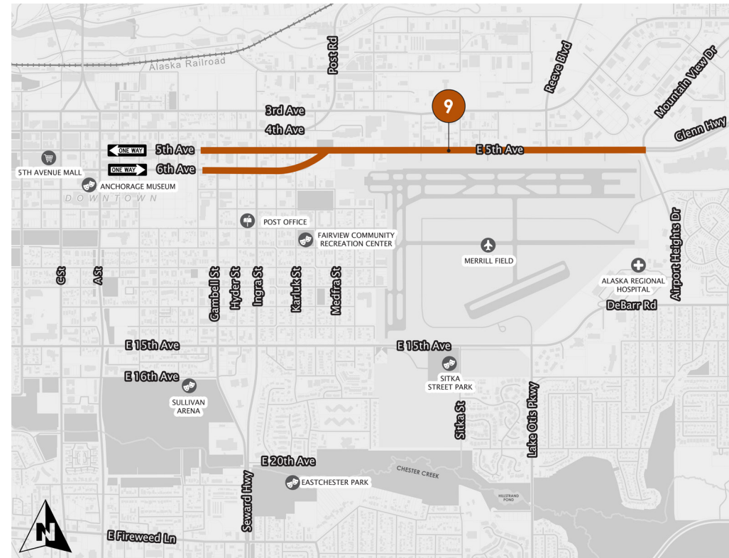
Figure 51: Phasing Plan: Phase 9—5 th -6 th Avenue Lane Drops and Complete Street
