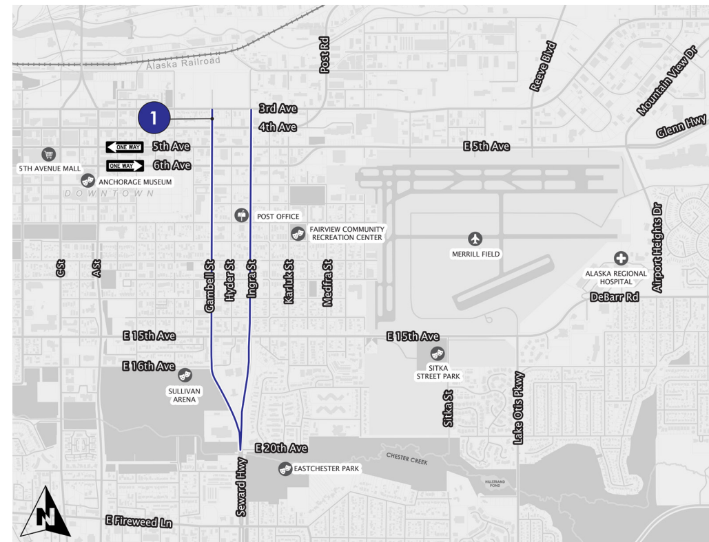
Figure 28: Phasing Plan: Phase 1 (Ingra-Gambell Couplet Lane Drops)
